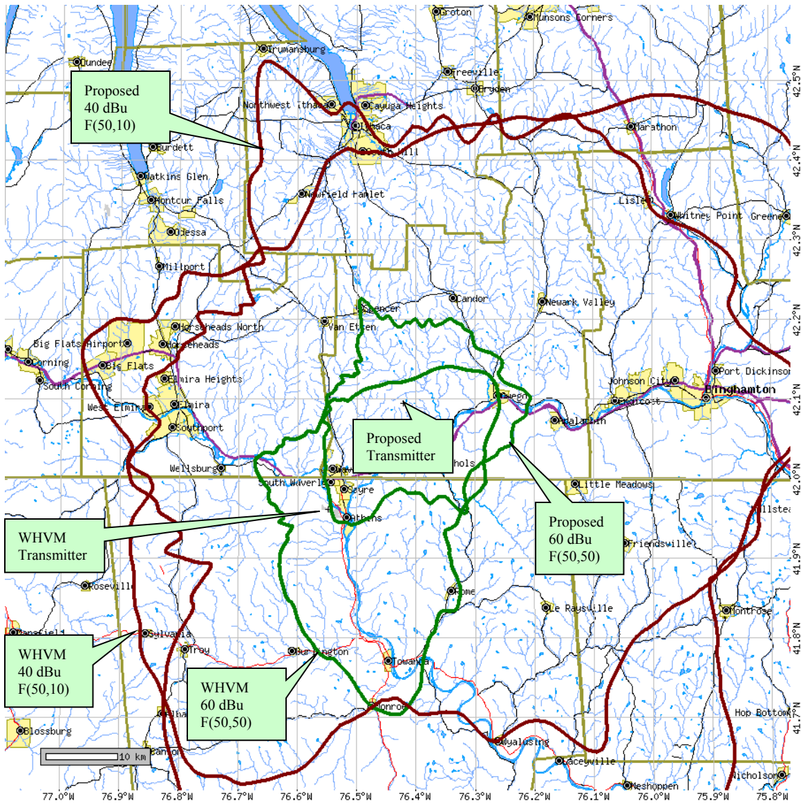
Figure 4. Predicted §73.509 contour protection in relation to WHVM (BLED-20070413AFA), channel 219A, ITHACA, NY.
